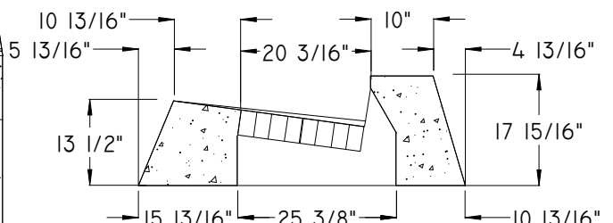
CONCRETE CURB TOP
