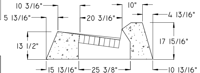
BITUMINOUS CURB TOP
