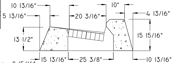
PARK CURB TOP
